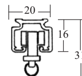
Track & Runner Dimentions
