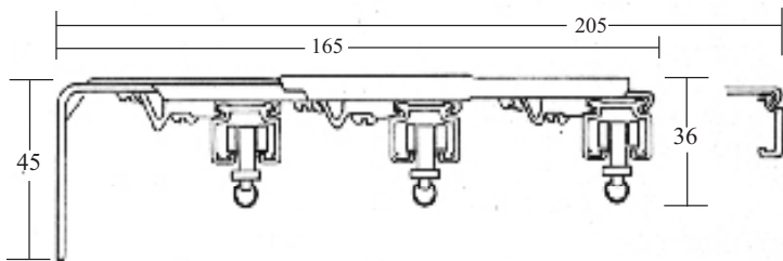
Triple Centre Support Bracket No 5259
