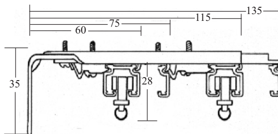
Centre Double Support Bracket No 5255S
