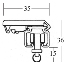
Small Ceiling Bracket No 5253
