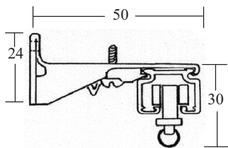
Fixed 50mm Projection Bracket No 5252
