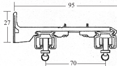
Fixed 95mm Projection Double Bracket No 5254
