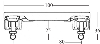
Double Ceiling Bracket No 5258
