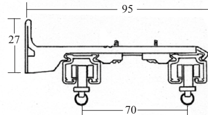
Fixed 95mm Projection Double Bracket No 5254
