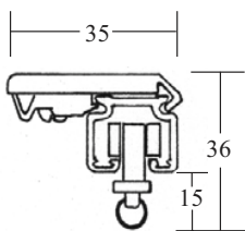
Small Ceiling Bracket No 5253
