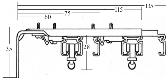
Centre Double Support Bracket No 5255S
