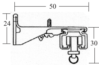
Fixed 50mm Projection Bracket No 5252
