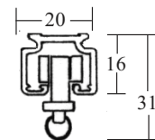
Track & Runner Dimentions
