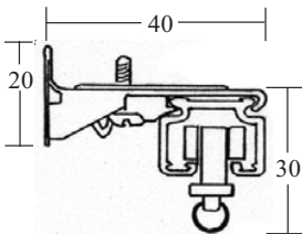
Fixed 40mm Projection Bracket No 5251
