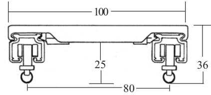
Double Ceiling Bracket No 5258
