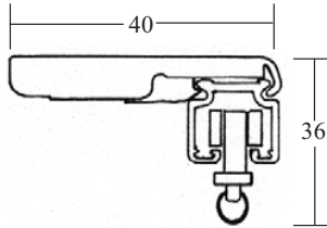
Large Ceiling Bracket No 5253L
