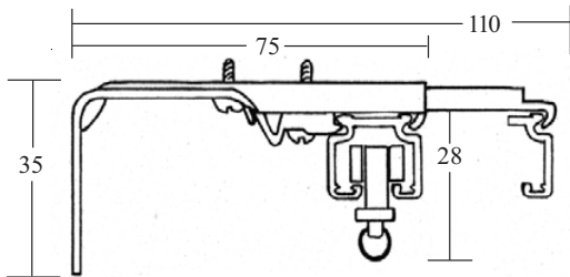
Centre Single Support Bracket No 5255
