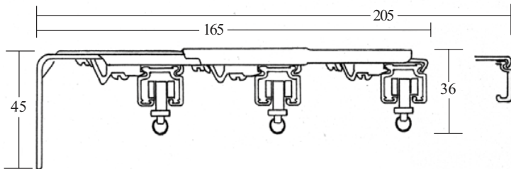
Triple Centre Support Bracket No 5259
