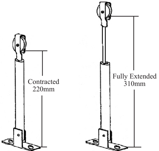
5375 Heavy Duty Cord Tensioner
