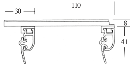
Double Ceiling Fix Bracket No 7358
