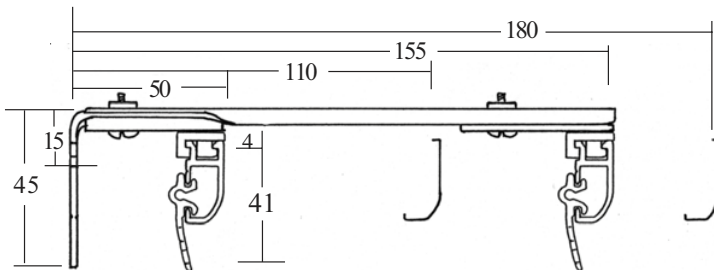
Double Centre Support Bracket Long No 7355L
