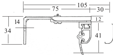
Single Ceiling Fix Bracket No 7353
