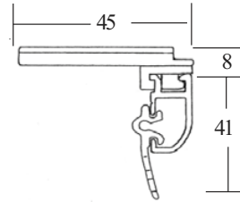
Ceiling Fixed Bracket No 7353A
