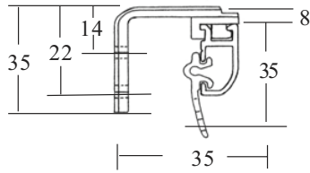
Fixed 35mm Projection Bracket No 7351
