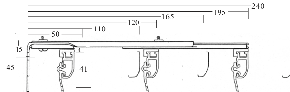
Triple Centre Support Bracket No 7359
