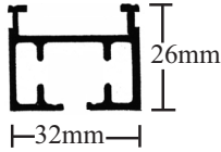
Series 80 Track Section Dimensions 8020
